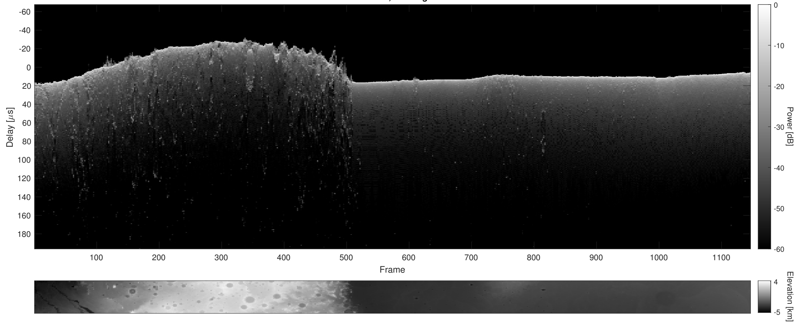
Orbit 12348, Cluttergram
