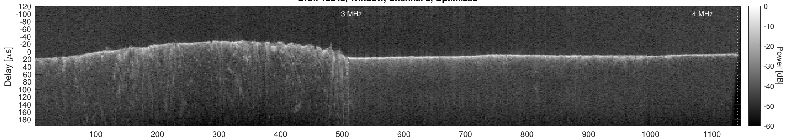
Orbit 12348, Cluttergram
