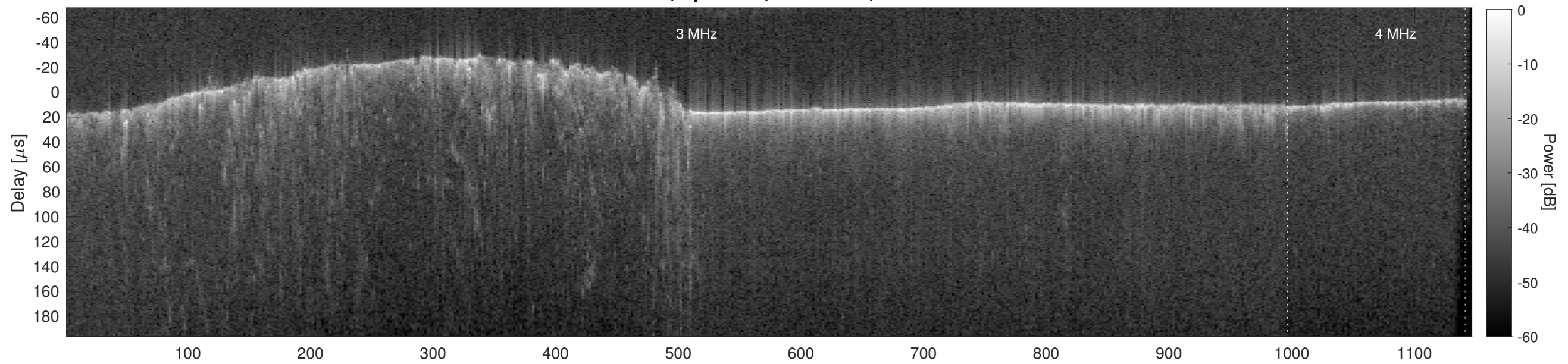
Orbit 12348, Cluttergram
