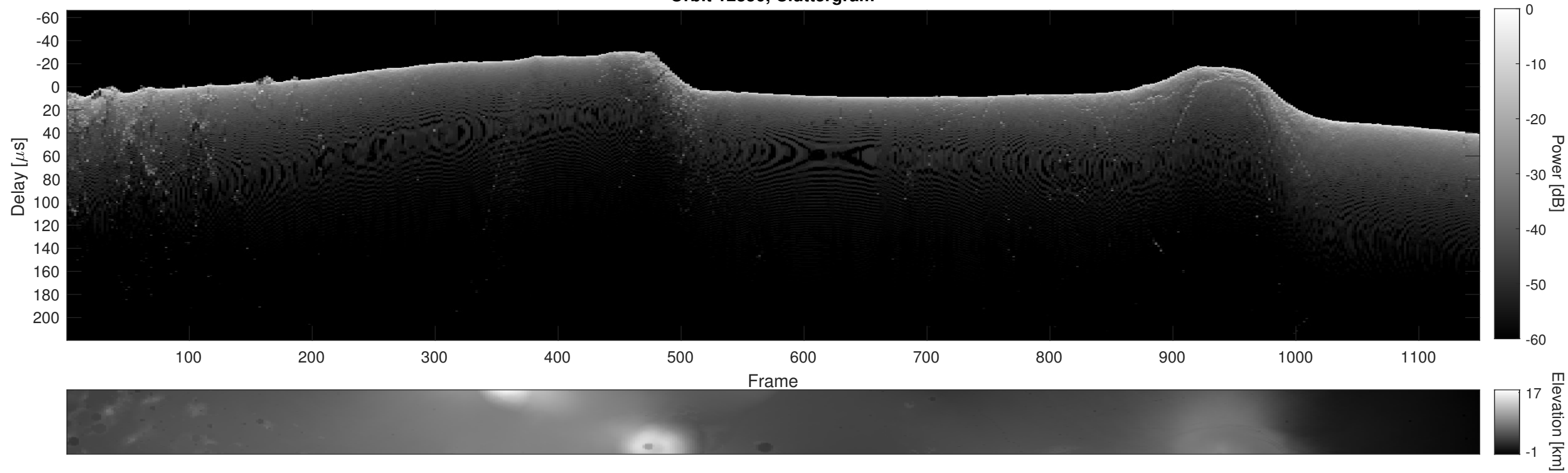
Orbit 12350, Cluttergram
