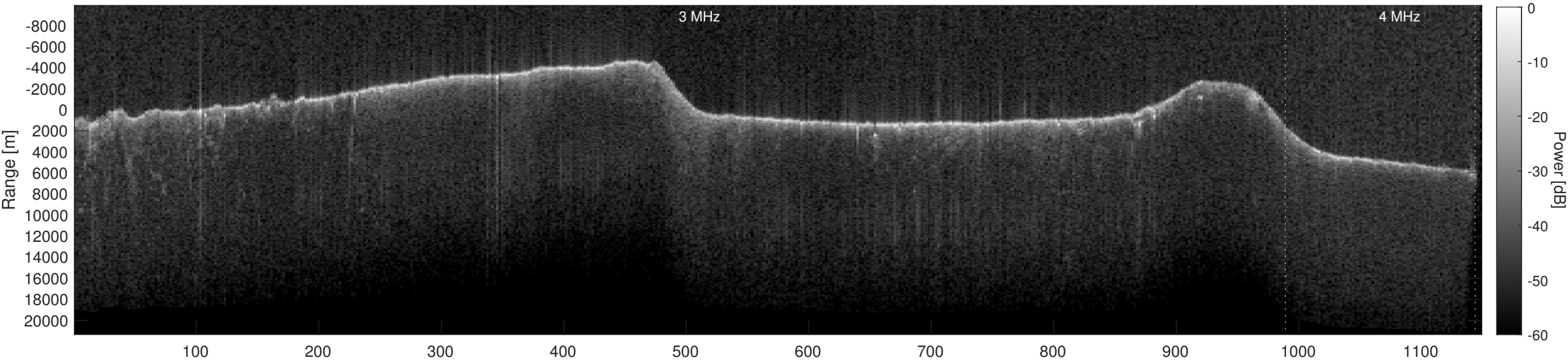
Orbit 12350, Depth-Corrected Cluttergram
