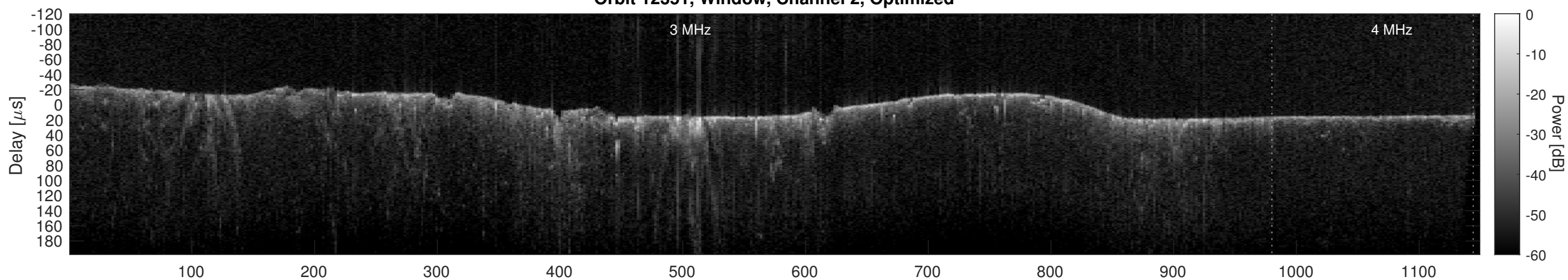
Orbit 12351, Cluttergram
