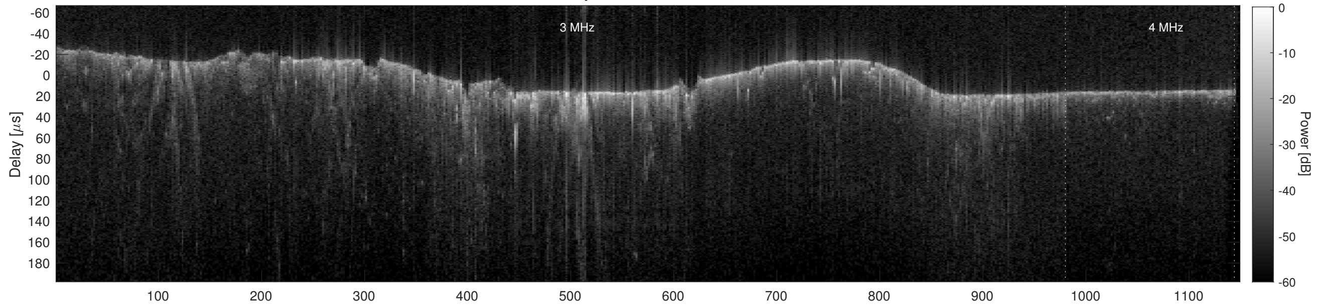
Orbit 12351, Cluttergram
