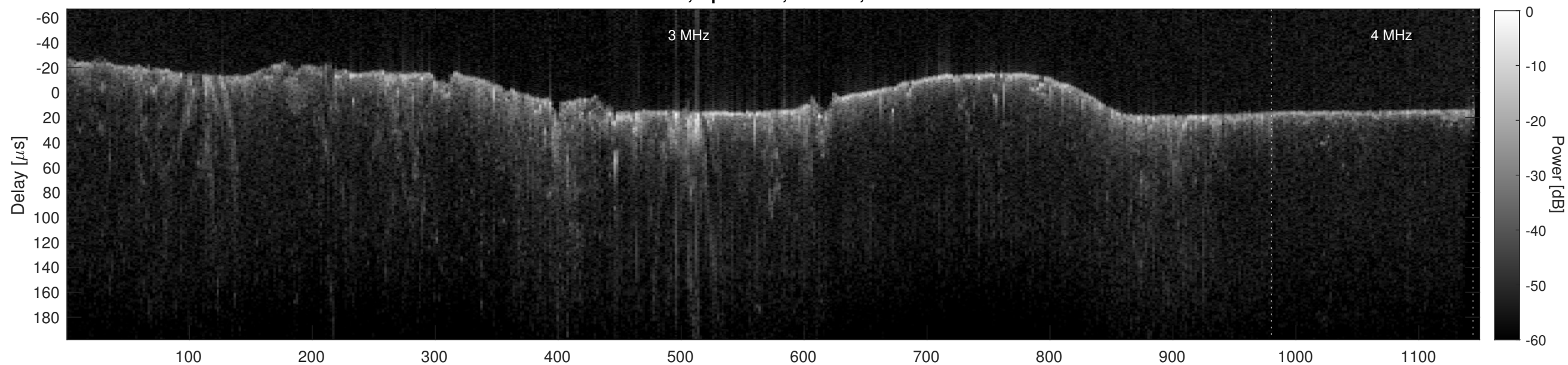
Orbit 12351, Cluttergram
