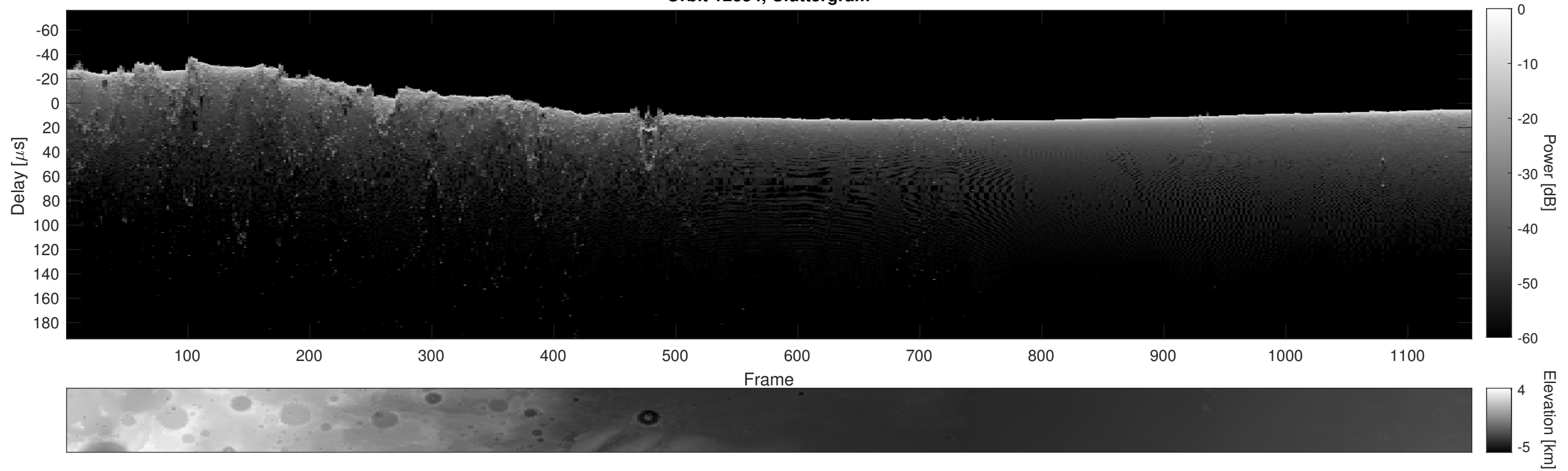
Orbit 12354, Cluttergram
