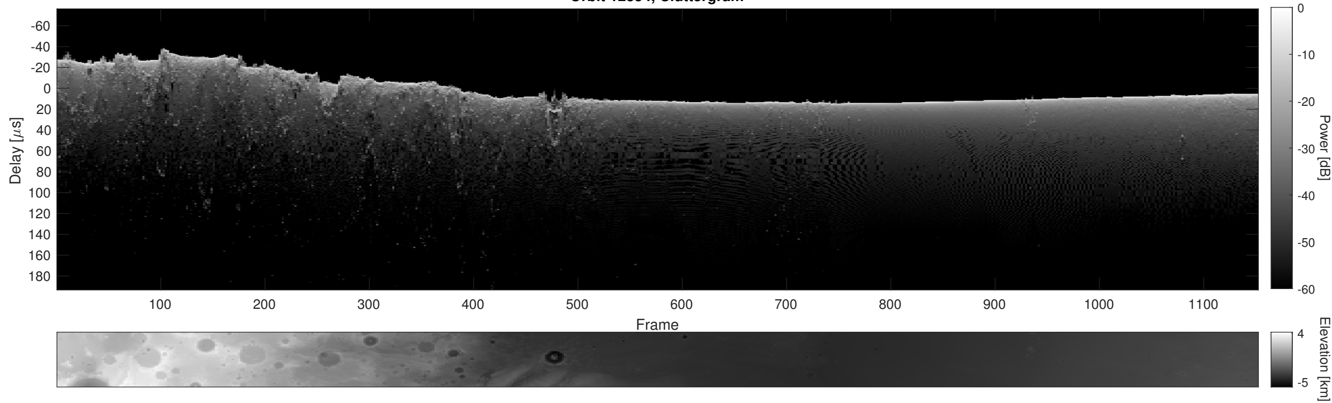
Orbit 12354, Cluttergram
