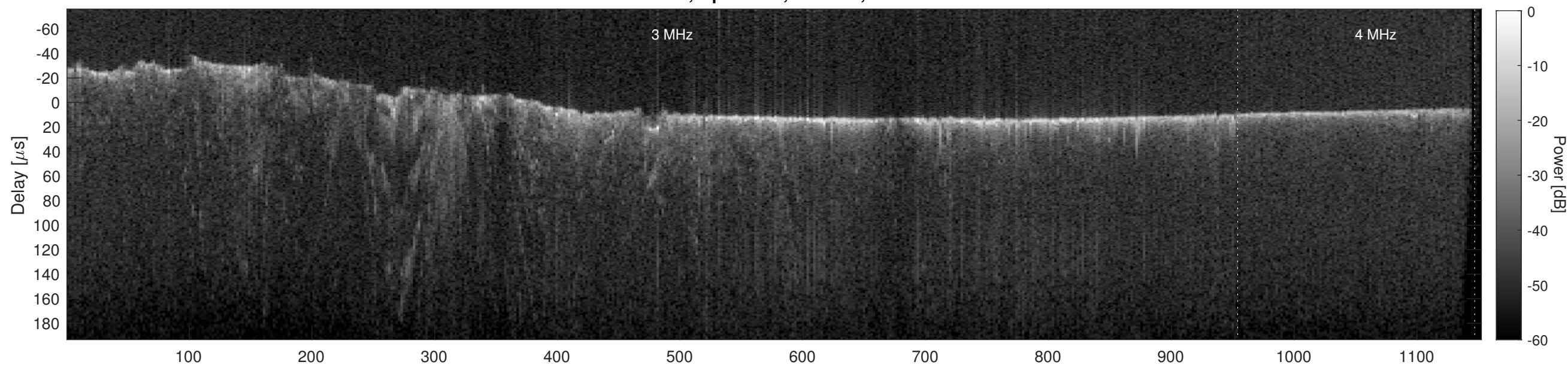
Orbit 12354, Cluttergram
