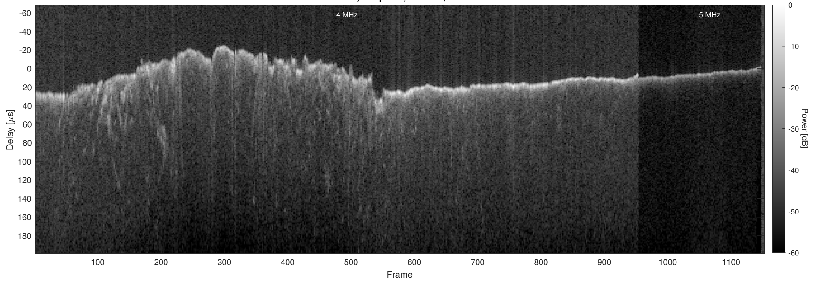
Orbit 12355, Chapman, Window, Channel 2
