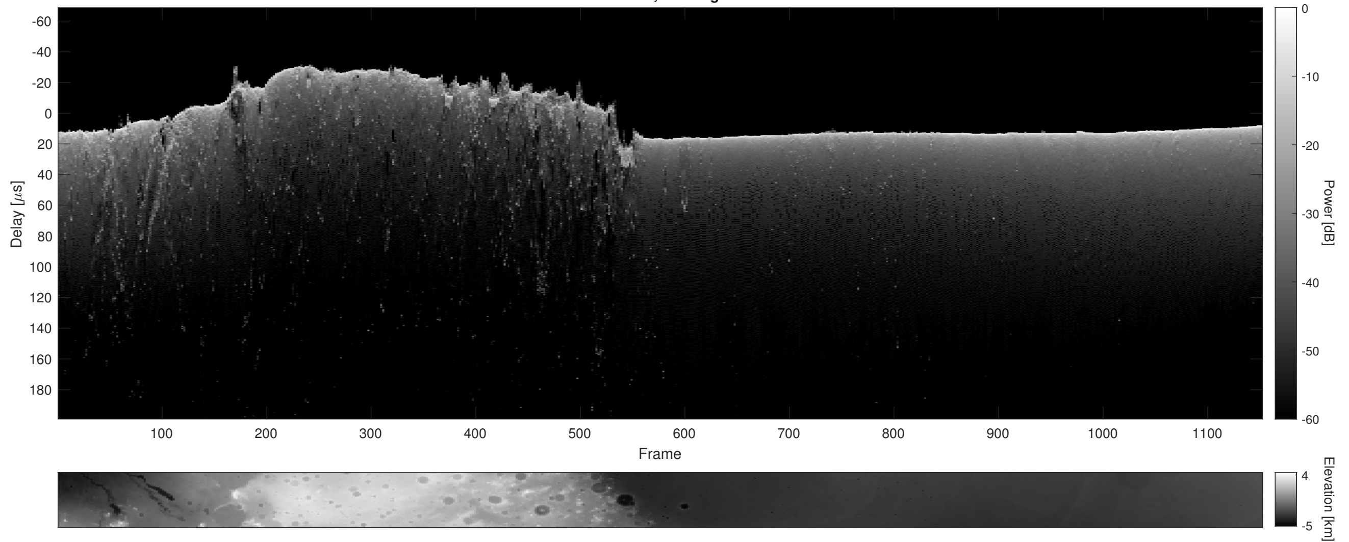
Orbit 12355, Cluttergram
