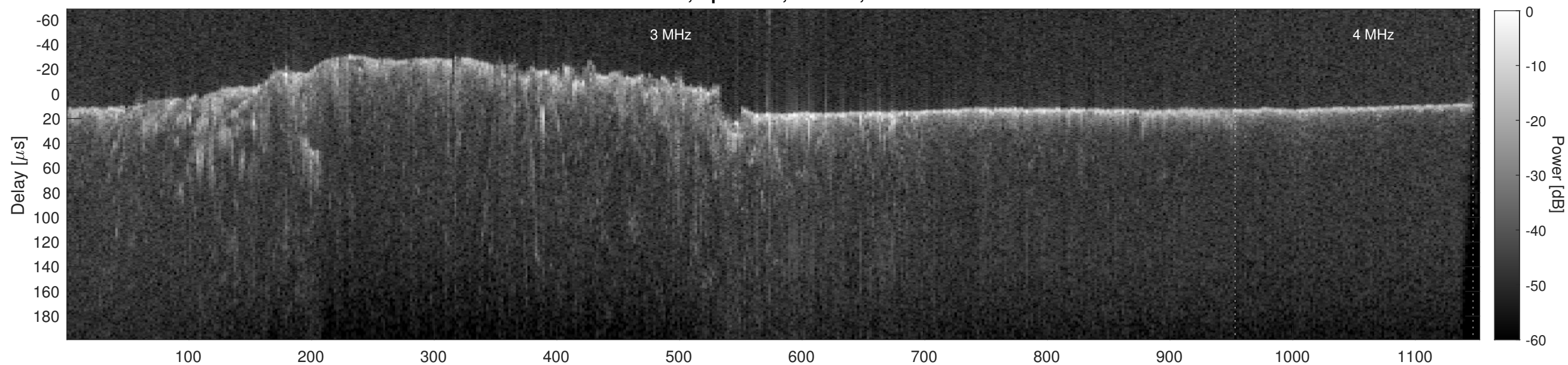
Orbit 12355, Cluttergram
