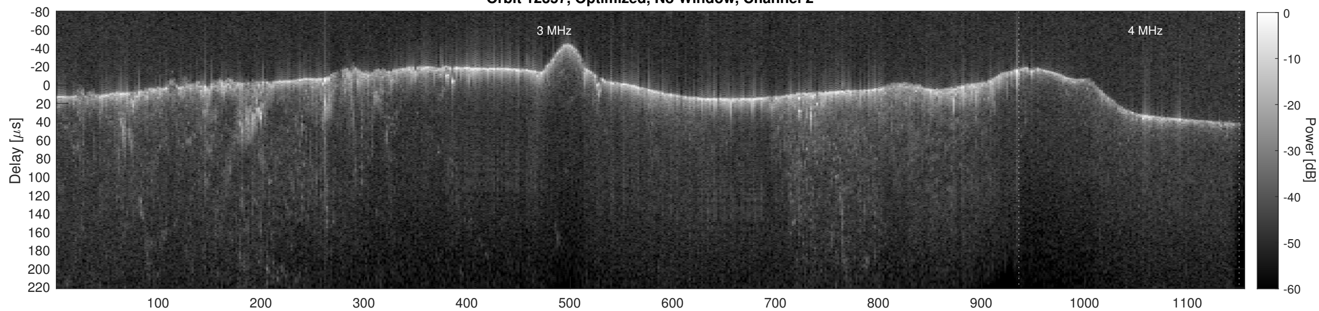
Orbit 12357, Cluttergram
