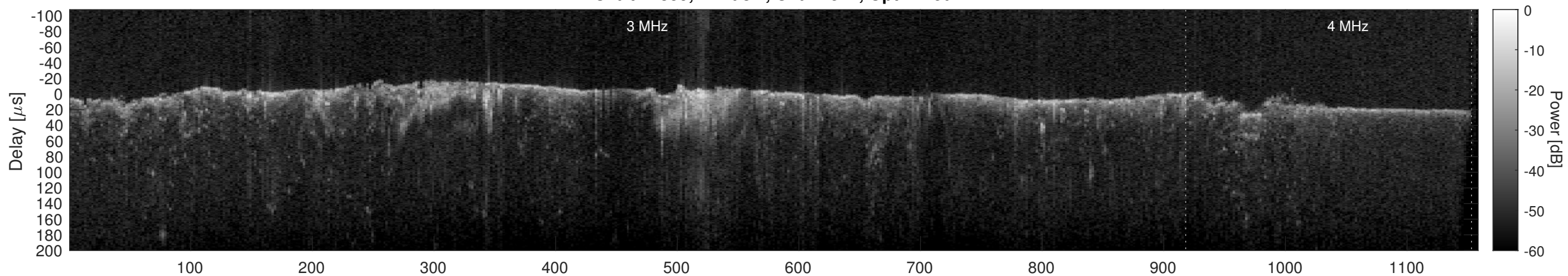
Orbit 12359, Cluttergram
