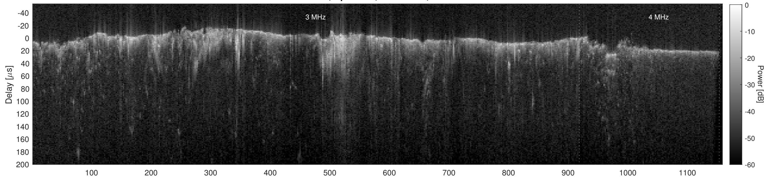
Orbit 12359, Cluttergram
