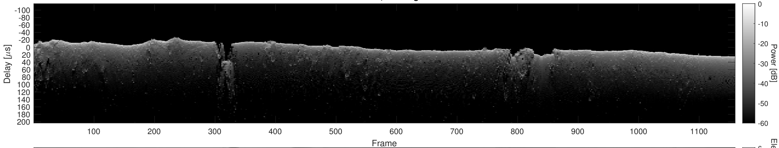
Orbit 12360, Cluttergram
