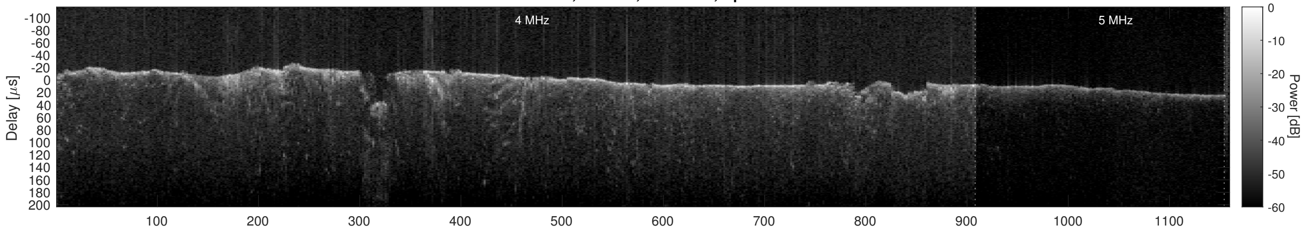
Orbit 12360, Cluttergram
