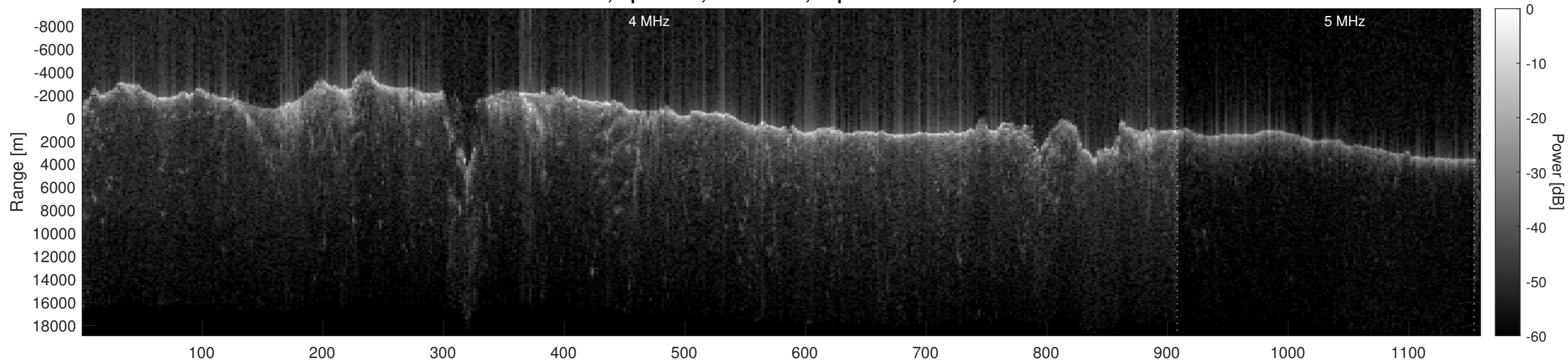
Orbit 12360, Optimized, No Window, Depth-Corrected, Channel 2
