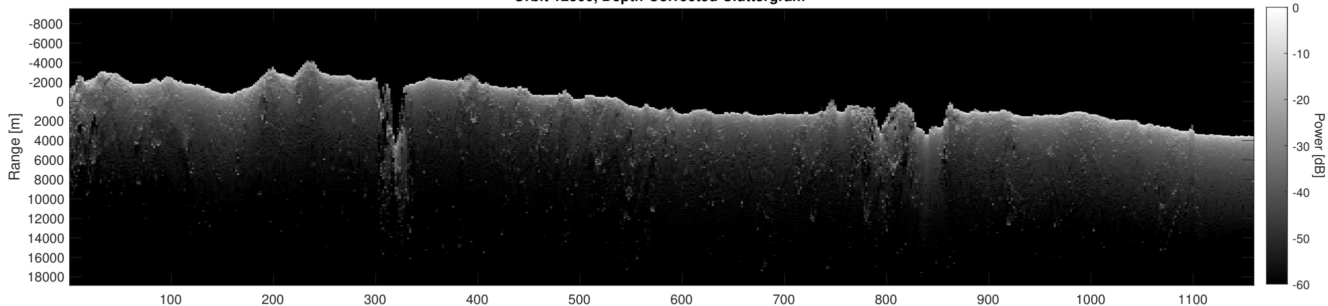
Orbit 12360, Depth-Corrected Cluttergram
