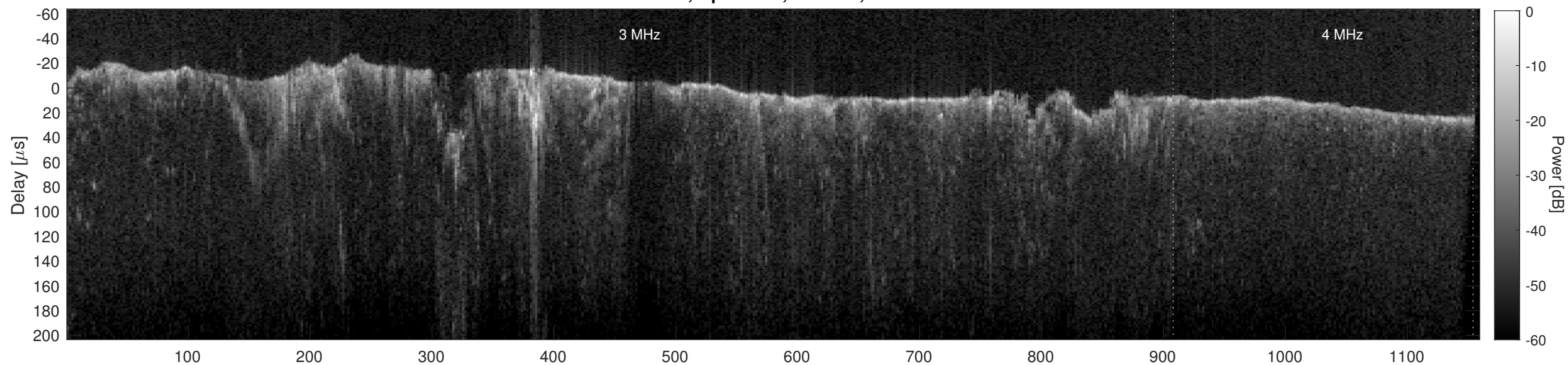
Orbit 12360, Cluttergram
