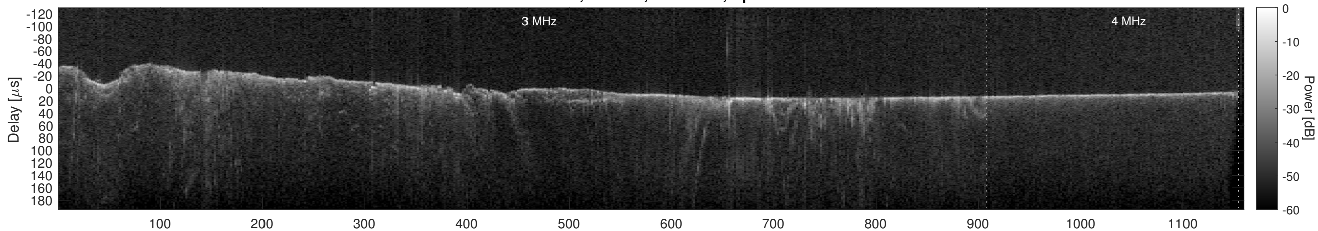
Orbit 12361, Cluttergram
