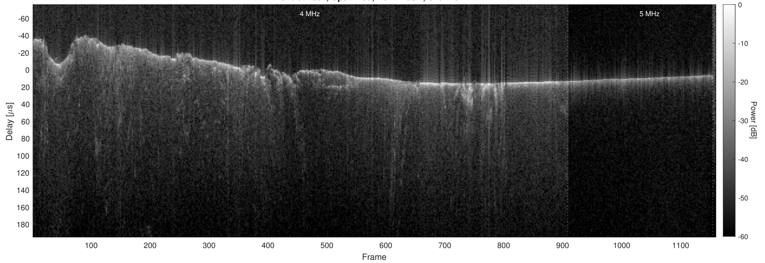
Orbit 12361, Optimized, No Window, Channel 2
