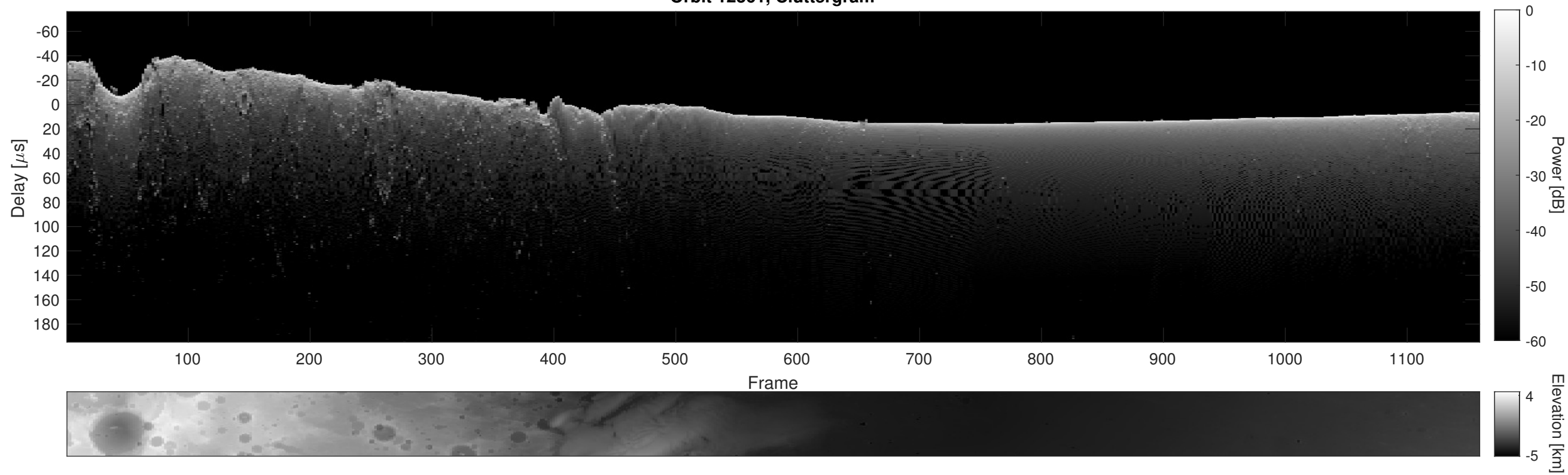
Orbit 12361, Cluttergram
