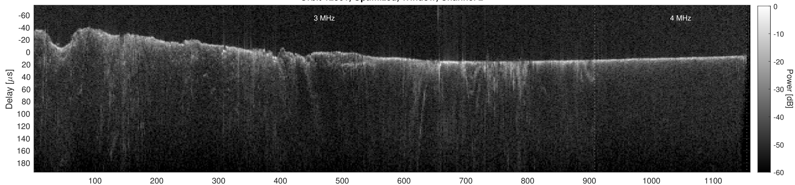
Orbit 12361, Cluttergram
