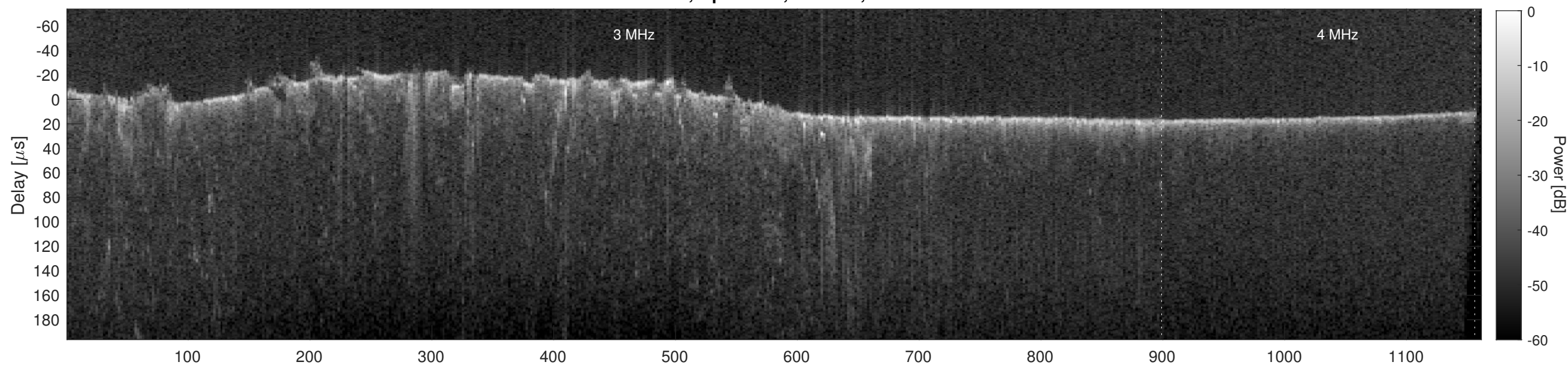
Orbit 12362, Cluttergram
