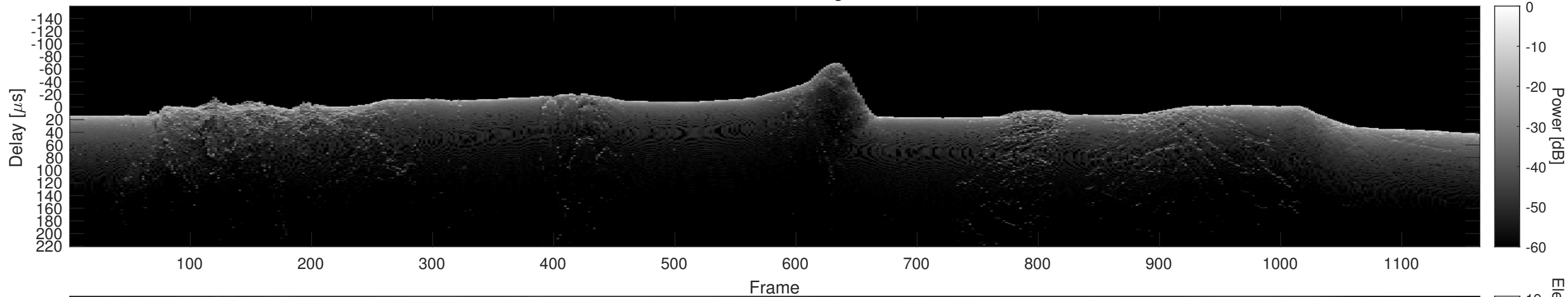
Orbit 12364, Cluttergram
