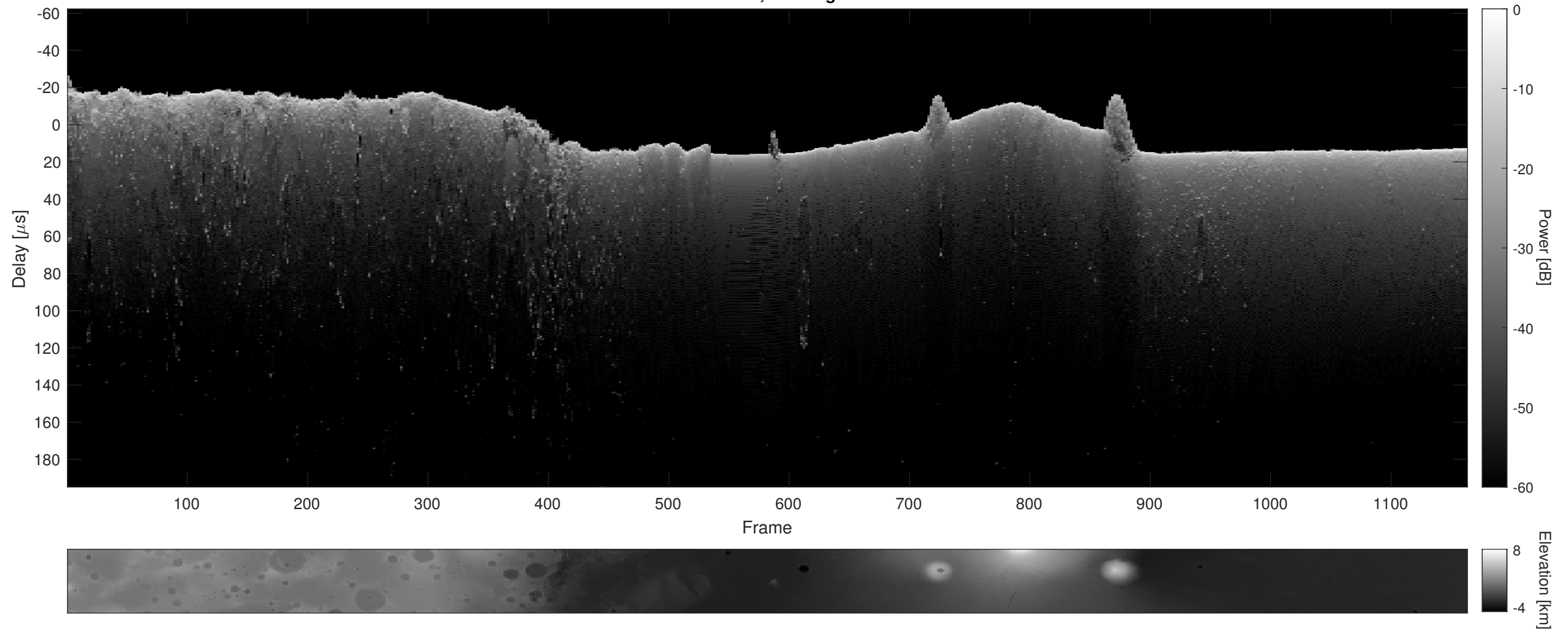
Orbit 12365, Cluttergram
