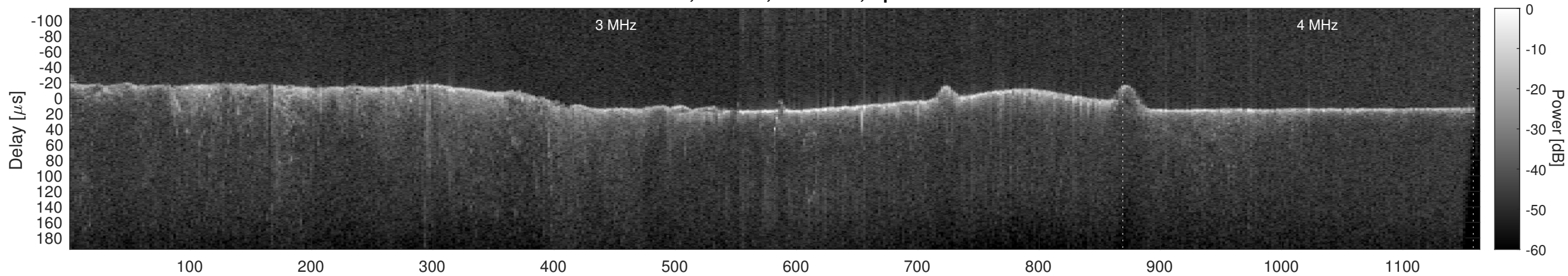
Orbit 12365, Cluttergram
