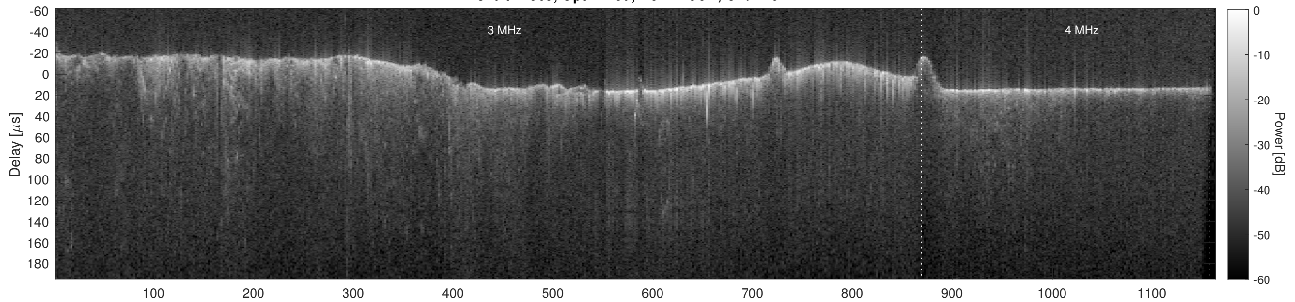
Orbit 12365, Cluttergram
