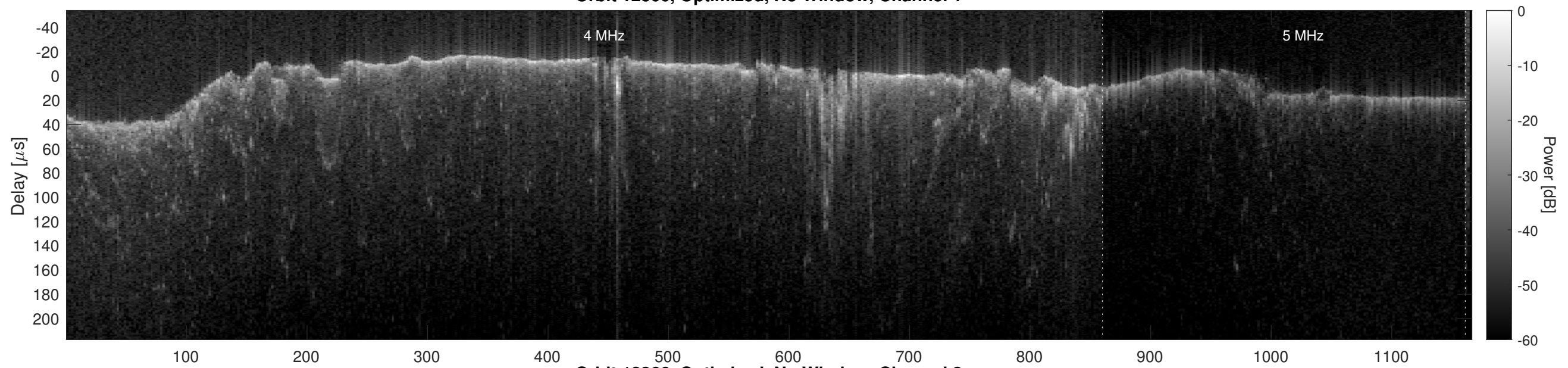
Orbit 12366, Optimized, No Window, Channel 2
