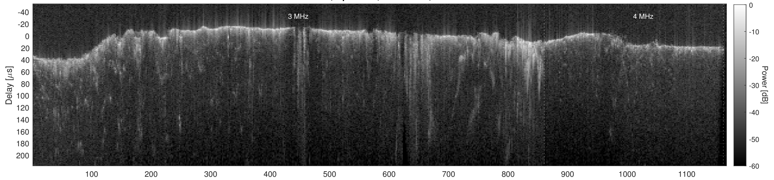
Orbit 12366, Cluttergram
