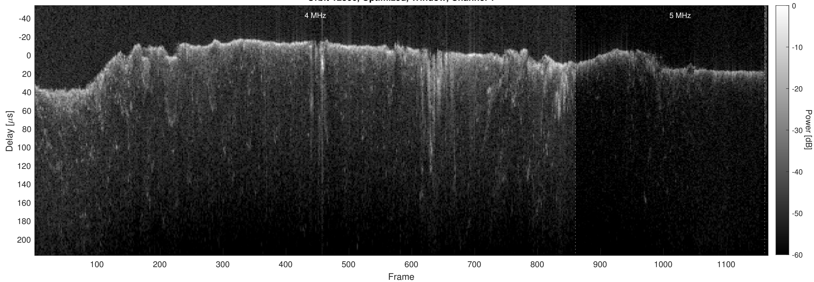
Orbit 12366, Optimized, Window, Channel 2
