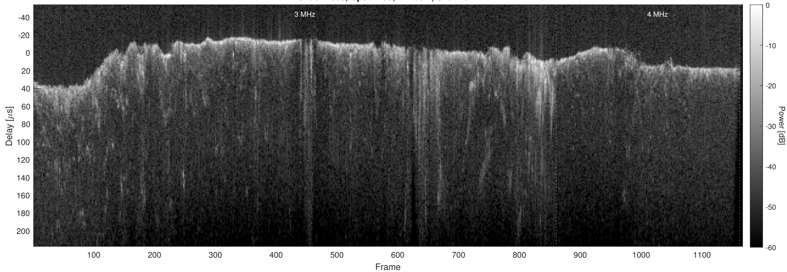
Orbit 12366, Optimized, Window, Channel 2
