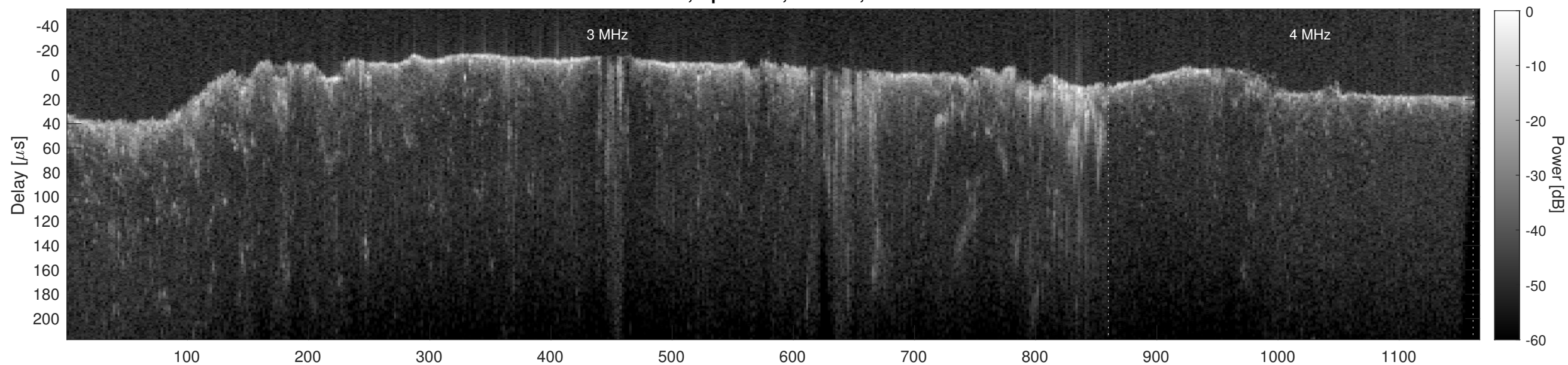
Orbit 12366, Cluttergram
