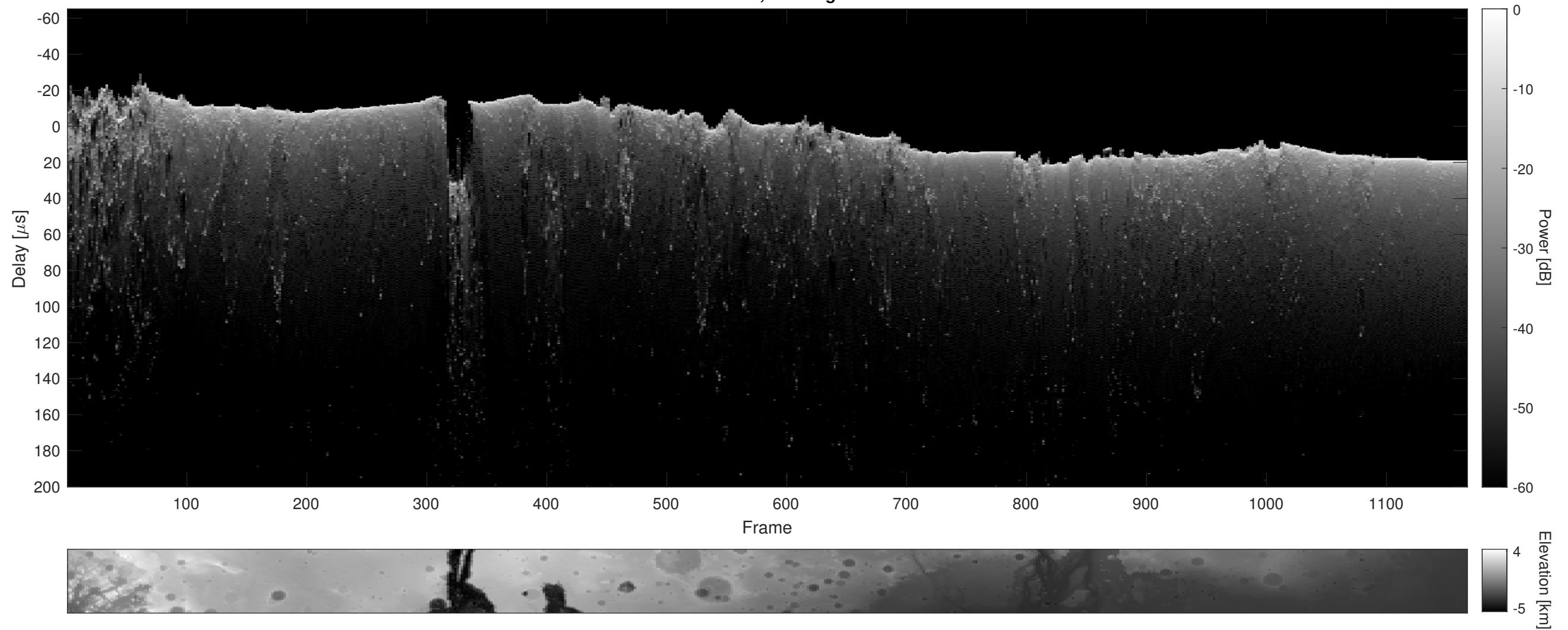
Orbit 12367, Cluttergram
