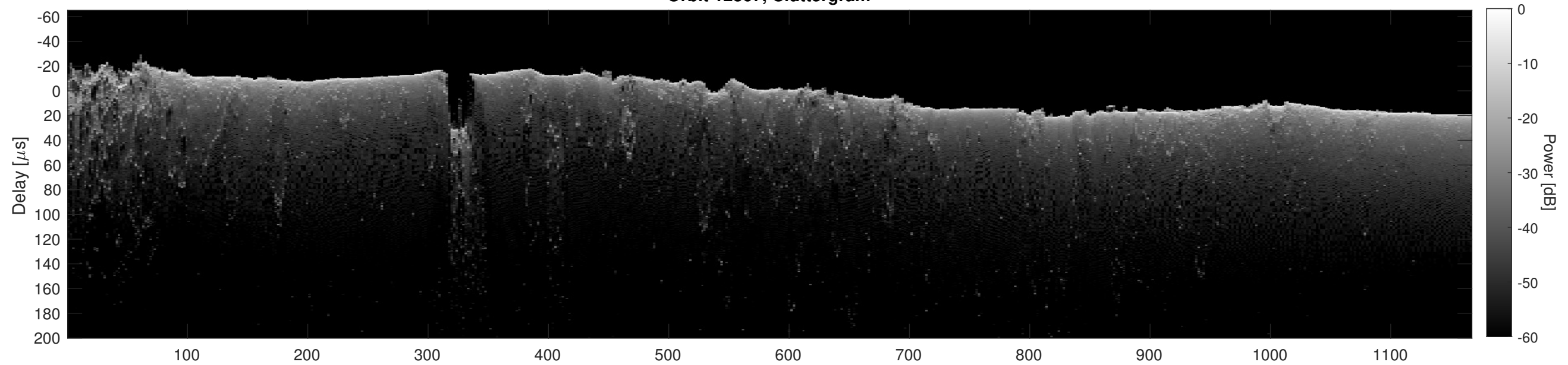
Orbit 12367, Cluttergram
