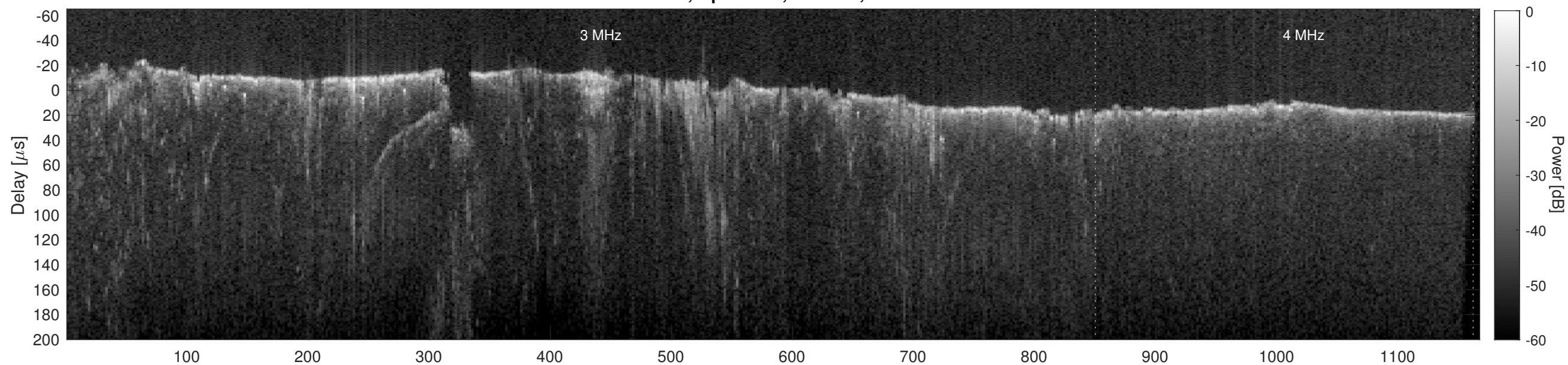
Orbit 12367, Cluttergram
