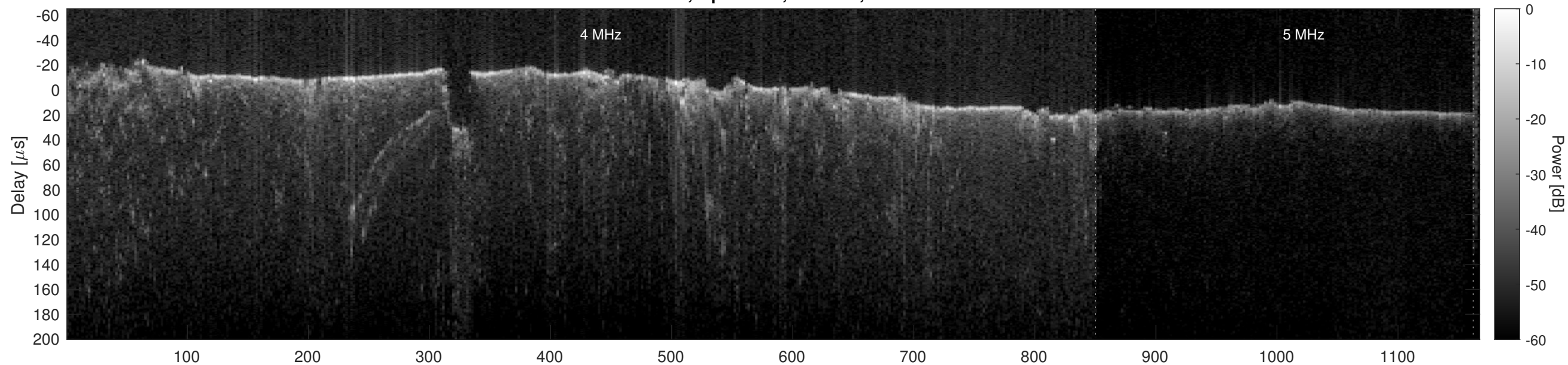
Orbit 12367, Optimized, Window, Channel 2
