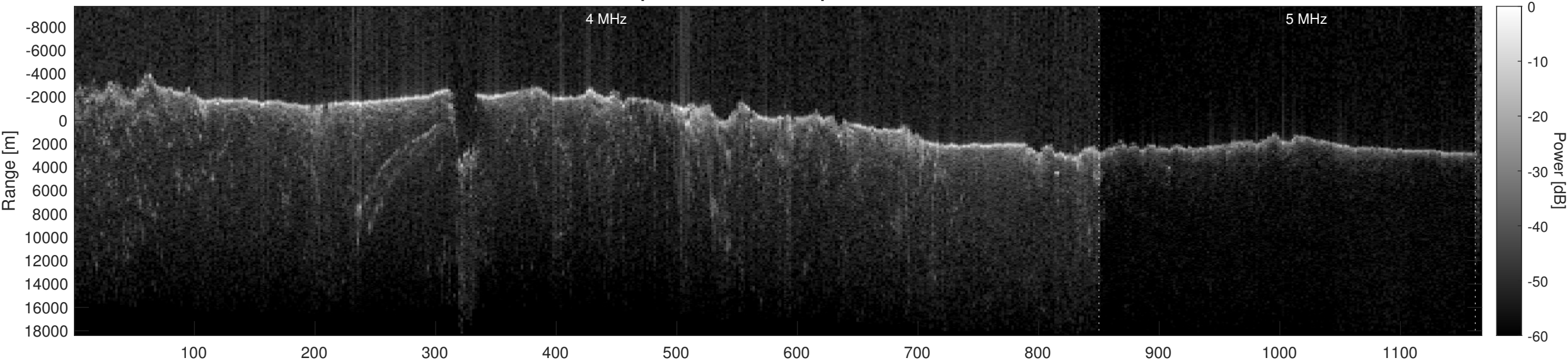
Orbit 12367, Optimized, Window, Depth-Corrected, Channel 2
