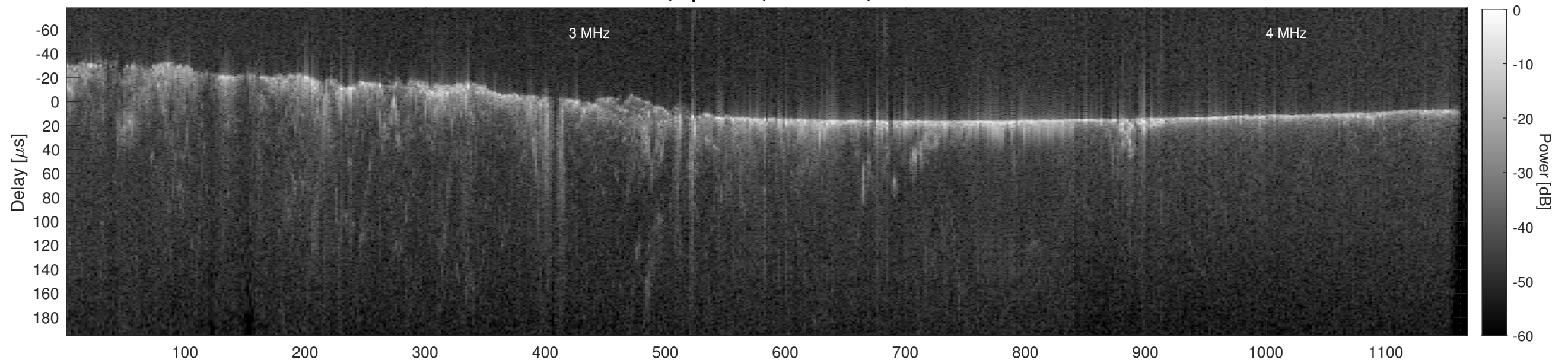
Orbit 12368, Cluttergram
