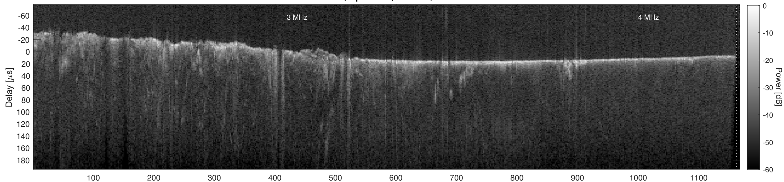
Orbit 12368, Cluttergram
