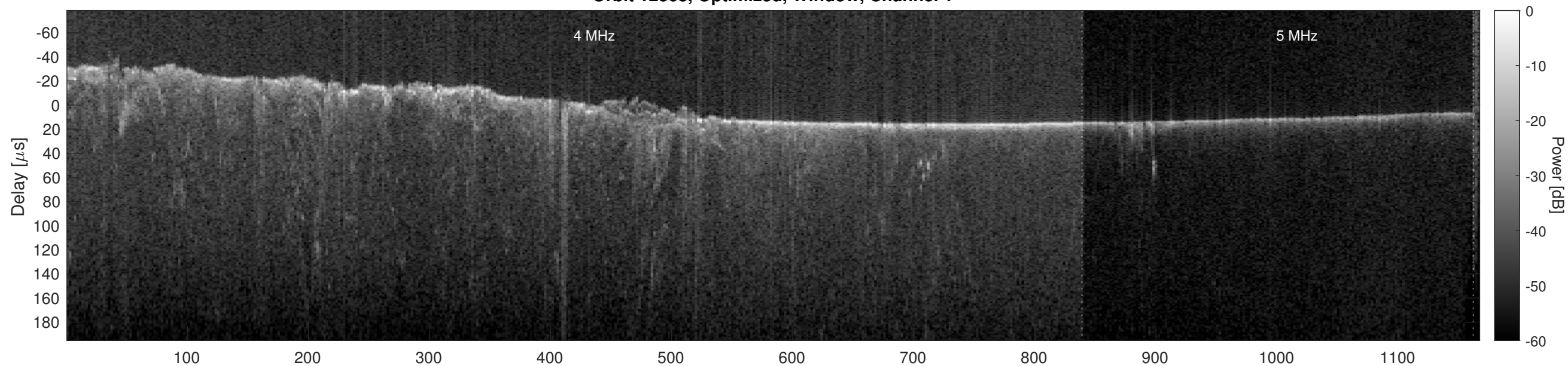
Orbit 12368, Optimized, Window, Channel 2
