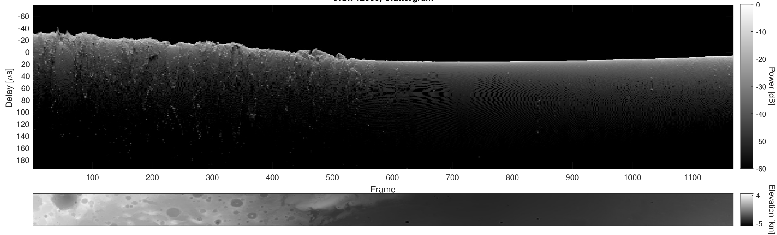
Orbit 12368, Cluttergram
