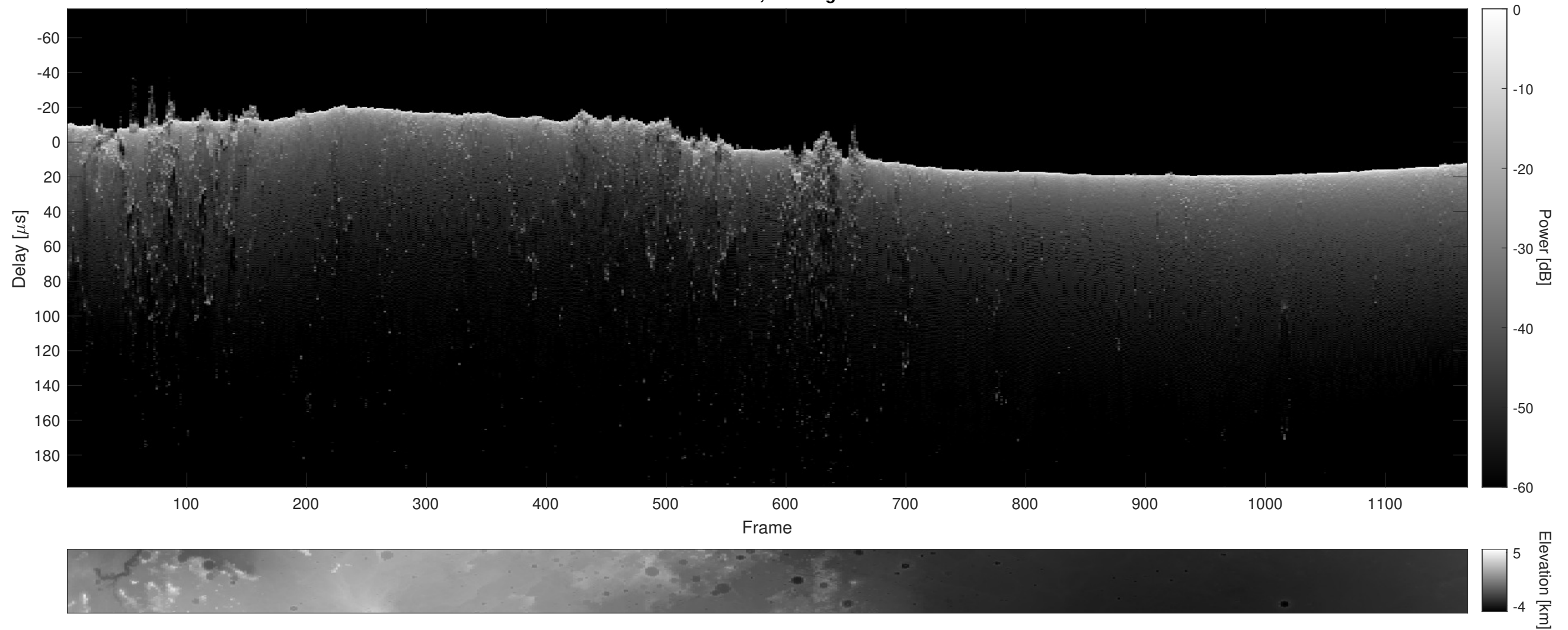
Orbit 12369, Cluttergram
