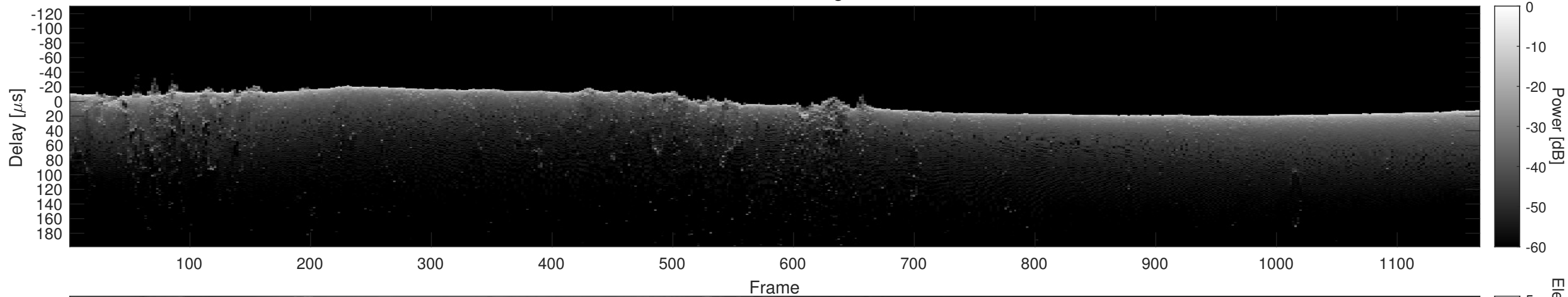
Orbit 12369, Cluttergram
