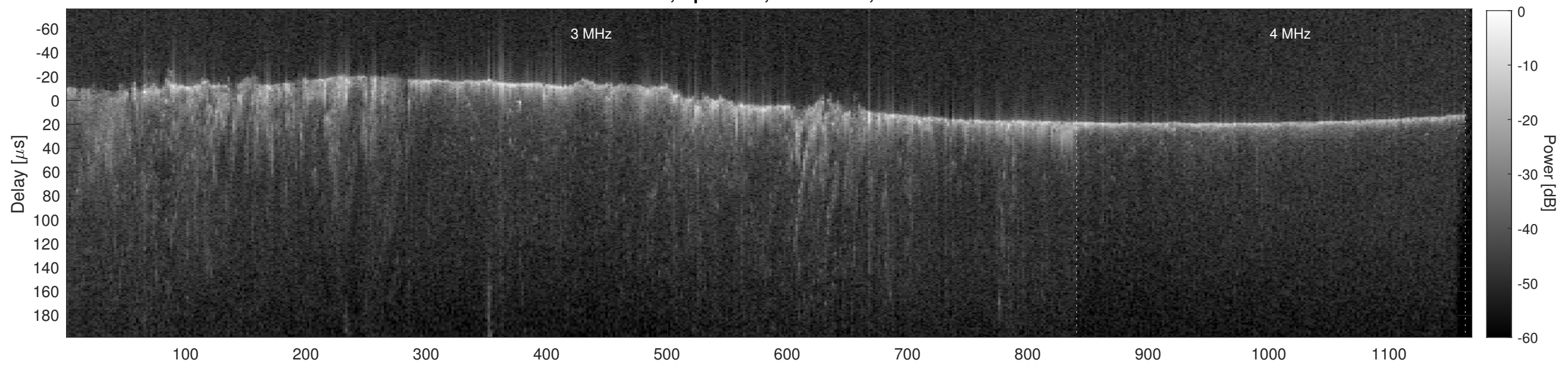
Orbit 12369, Cluttergram
