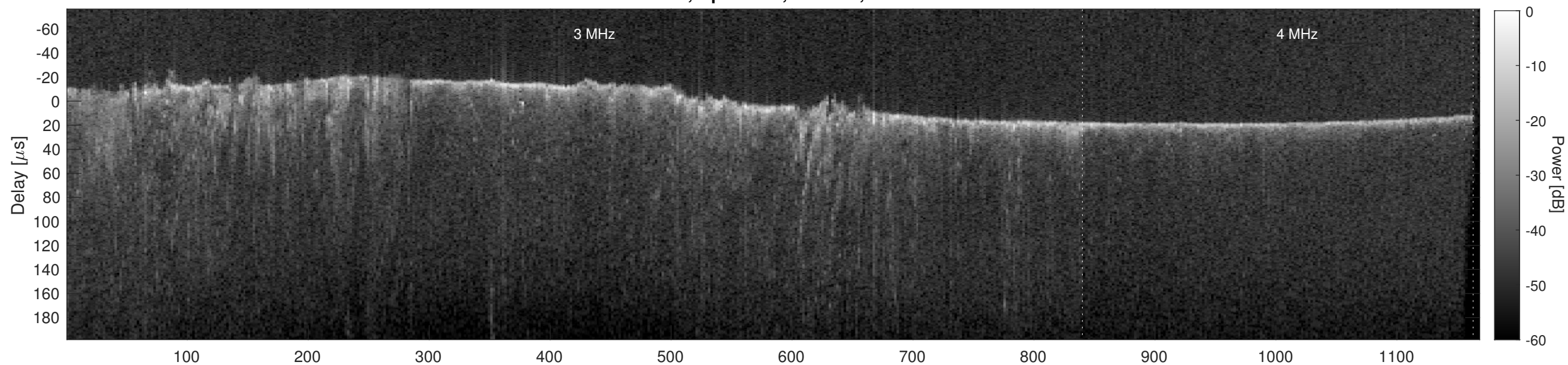
Orbit 12369, Cluttergram
