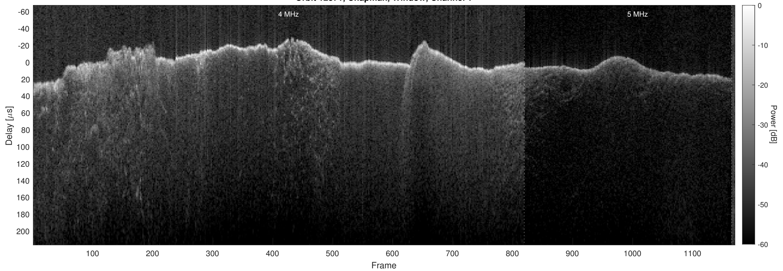
Orbit 12371, Chapman, Window, Channel 2
