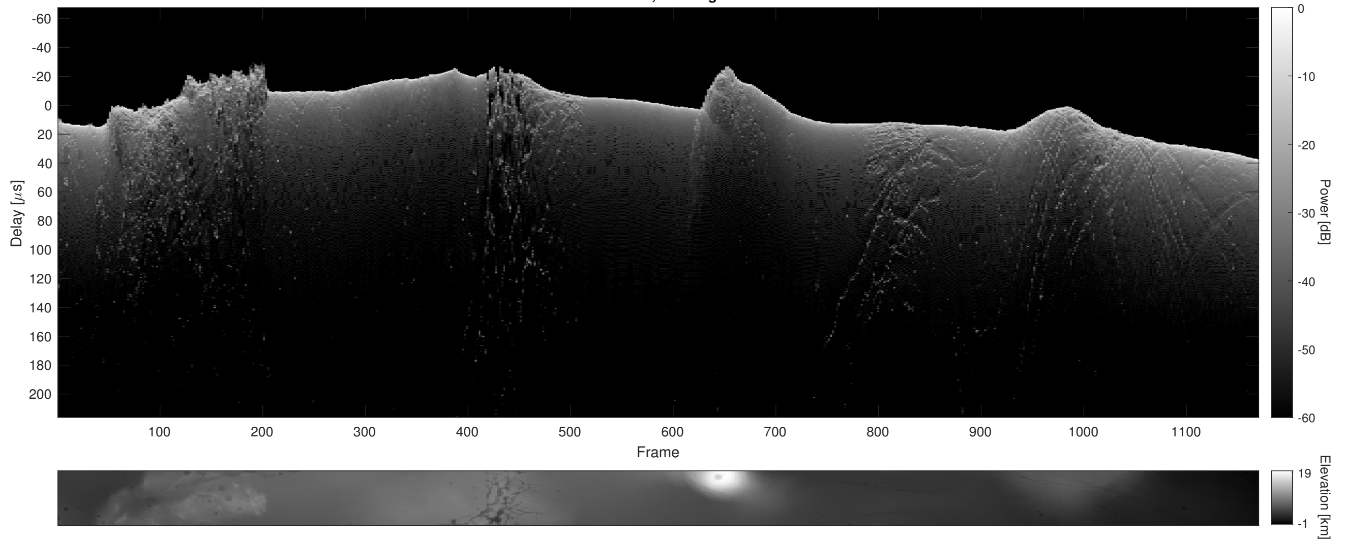
Orbit 12371, Cluttergram
