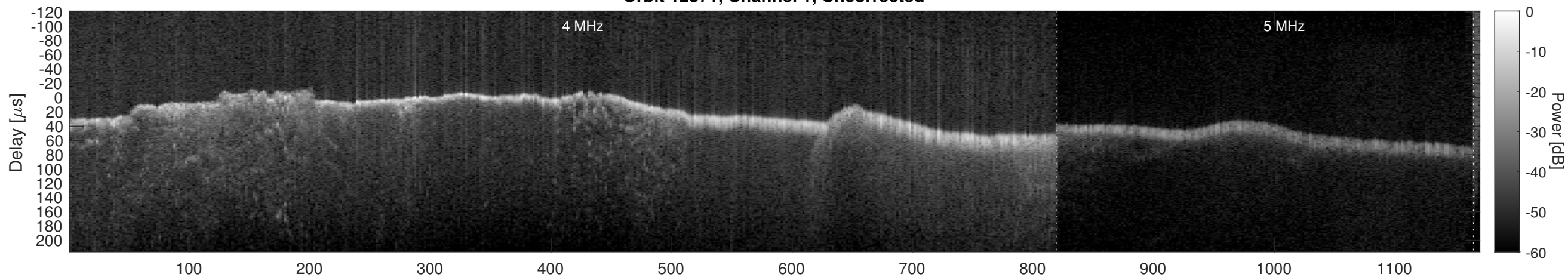
Orbit 12371, Window, Channel 1, Chapman
