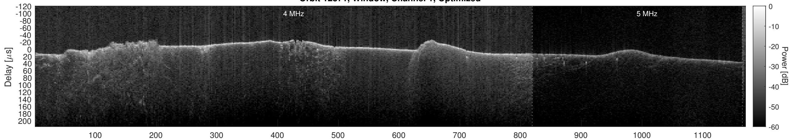
Orbit 12371, Cluttergram
