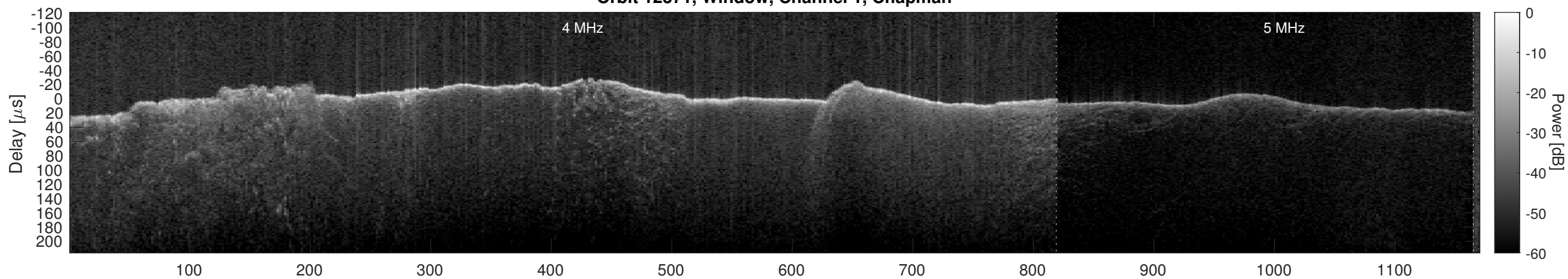
Orbit 12371, Window, Channel 1, Optimized
