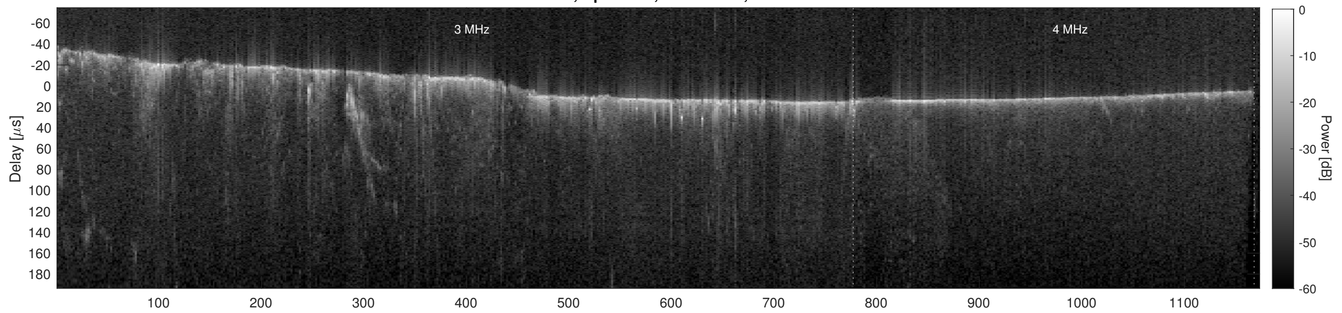
Orbit 12375, Cluttergram
