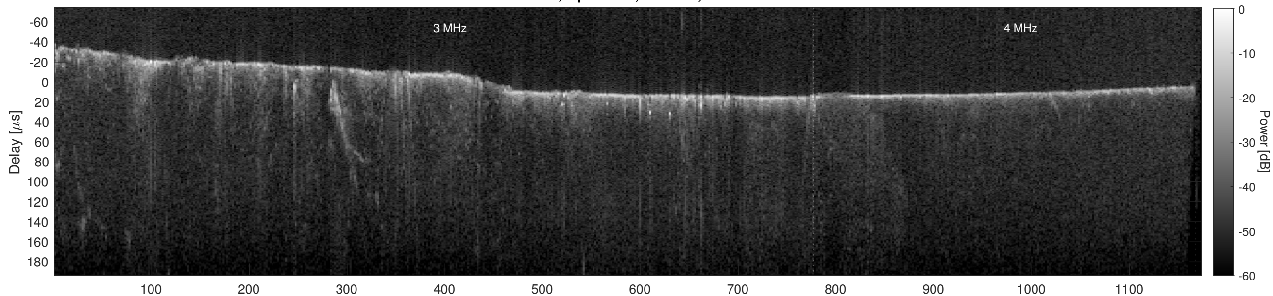
Orbit 12375, Cluttergram
