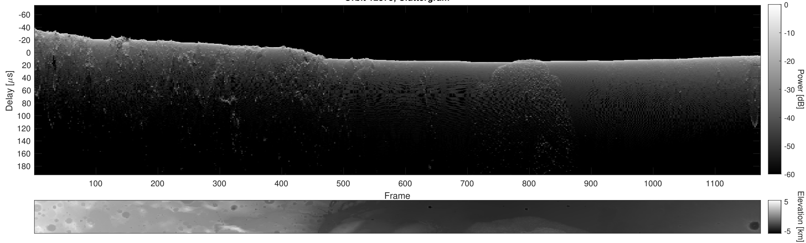
Orbit 12375, Cluttergram
