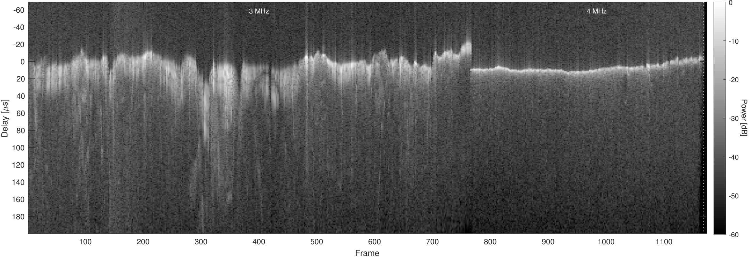
Orbit 12376, Chapman, No Window, Channel 2
