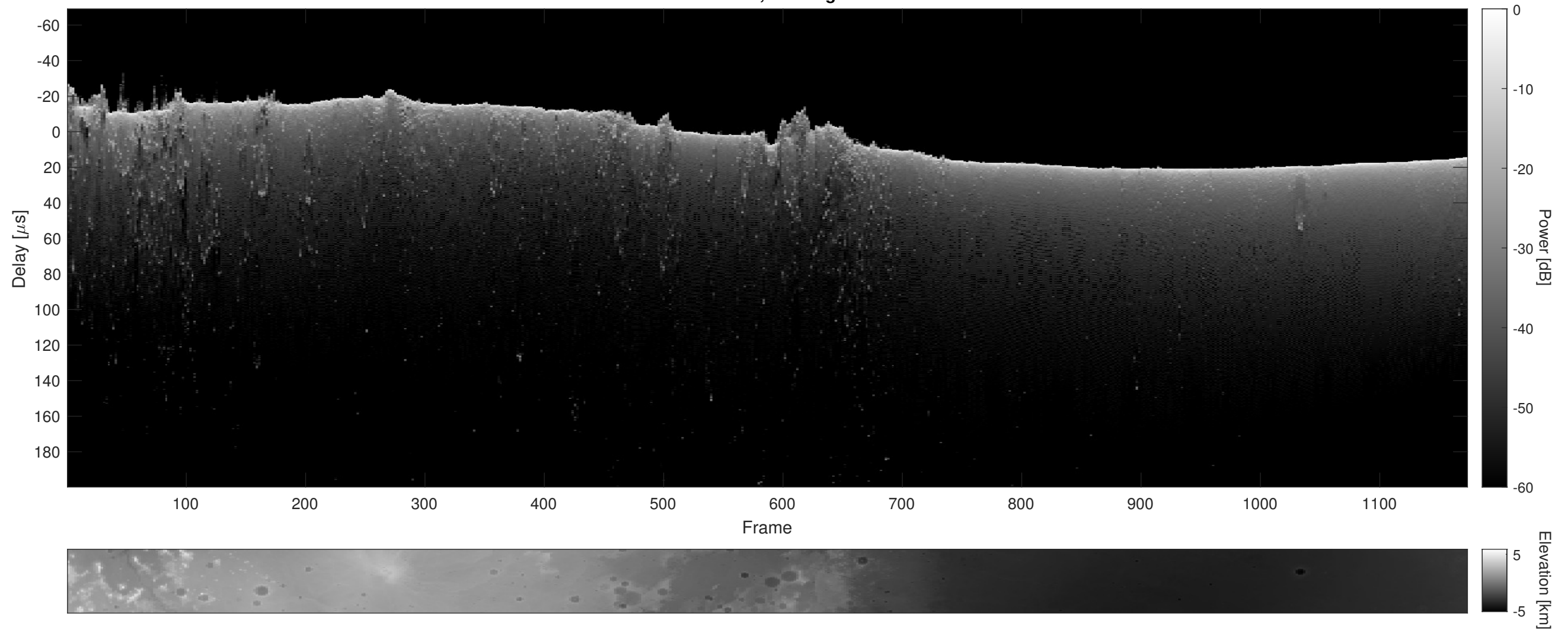
Orbit 12376, Cluttergram
