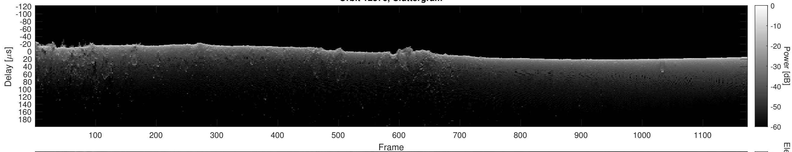
Orbit 12376, Cluttergram
