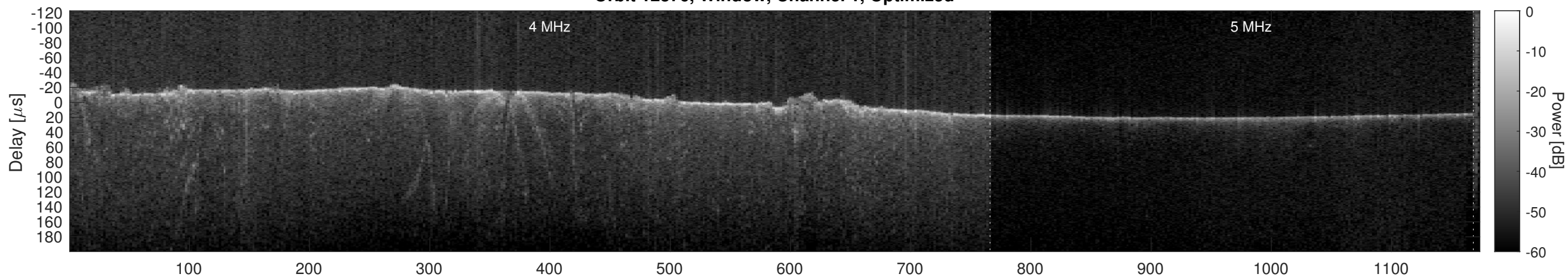
Orbit 12376, Cluttergram
