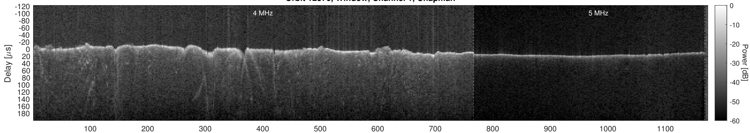
Orbit 12376, Window, Channel 1, Optimized
