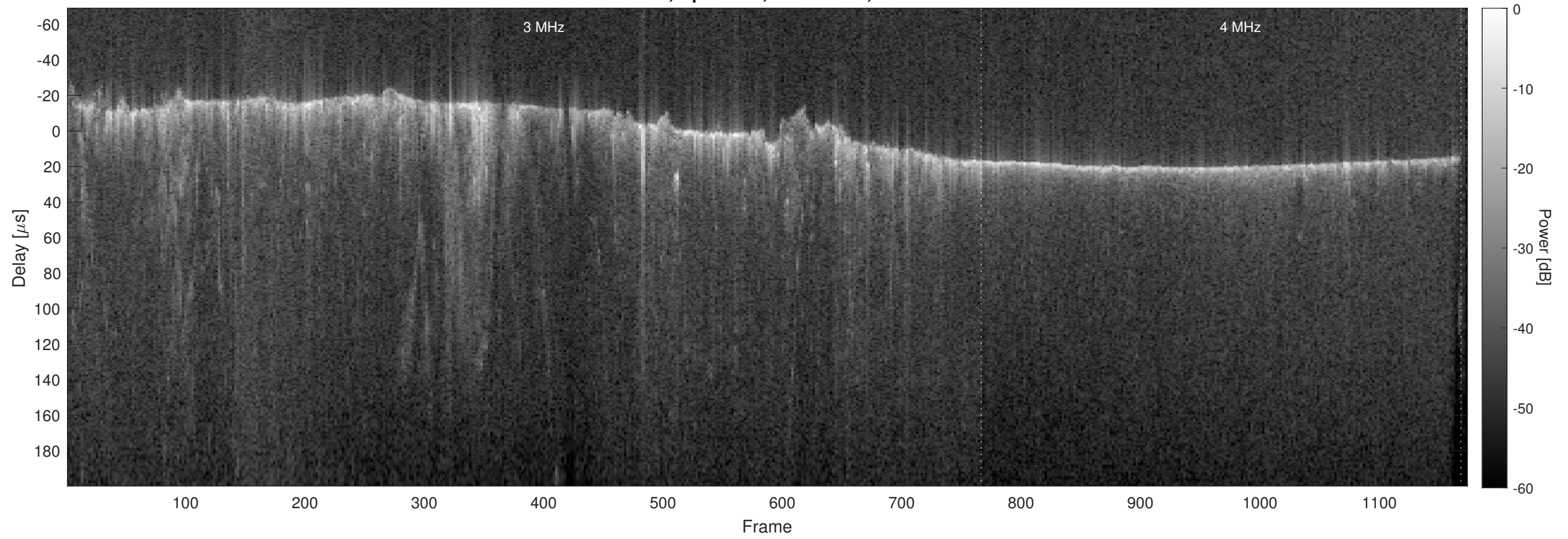
Orbit 12376, Optimized, No Window, Channel 2
