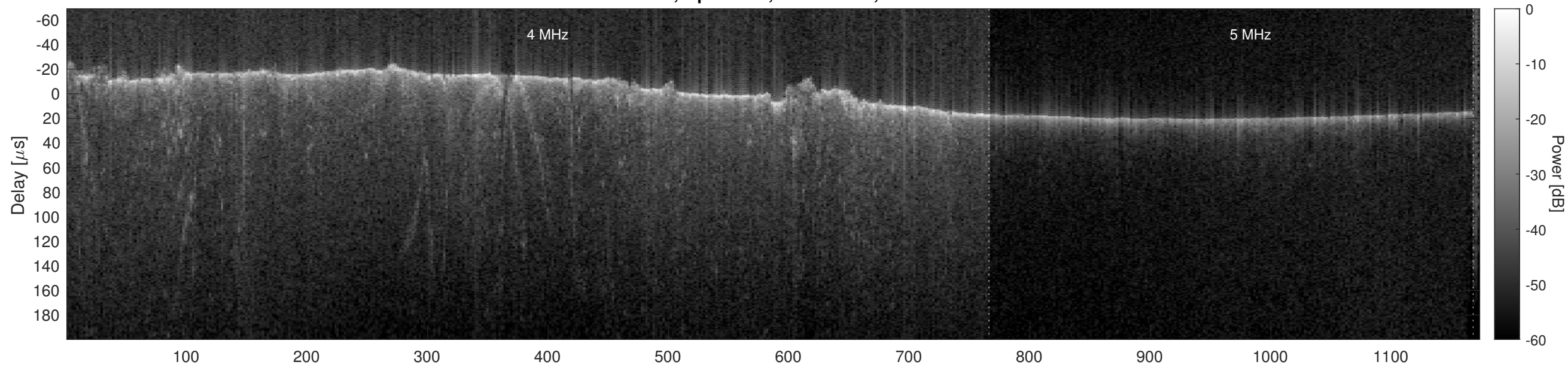
Orbit 12376, Optimized, No Window, Channel 2
